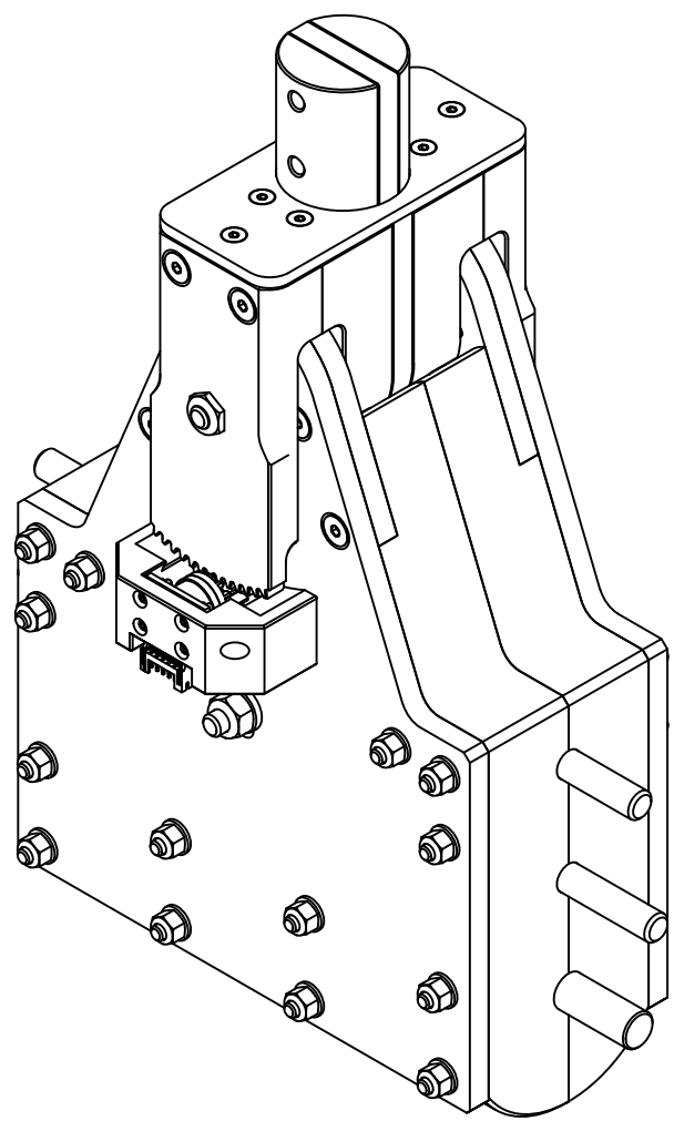
-100 ISO SCALE 1:2
