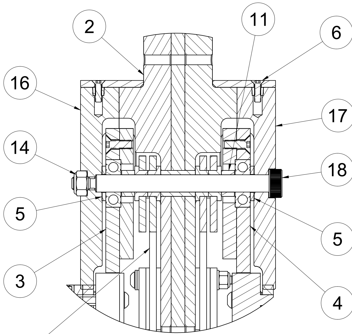
DETAIL E SCALE 1:1
