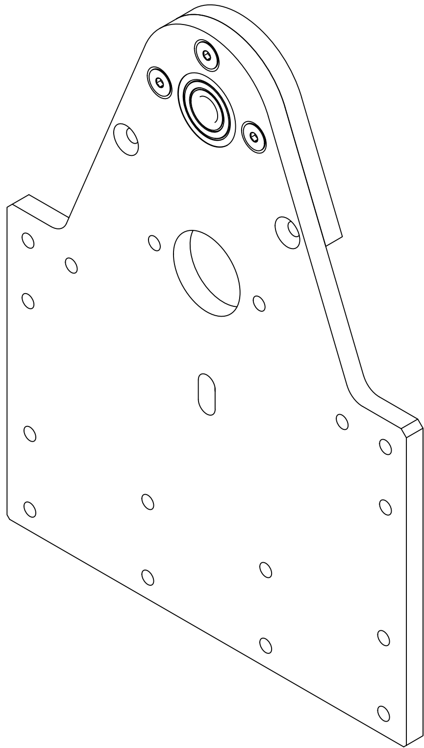
-119 ISO SCALE 1:1
